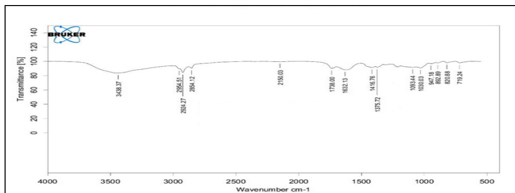
Fig. 9: FTIR Spectrum of Sodium Alginate
