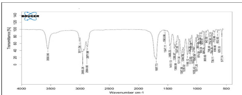
Fig. 8: FTIR Spectrum of Rosvastatin
