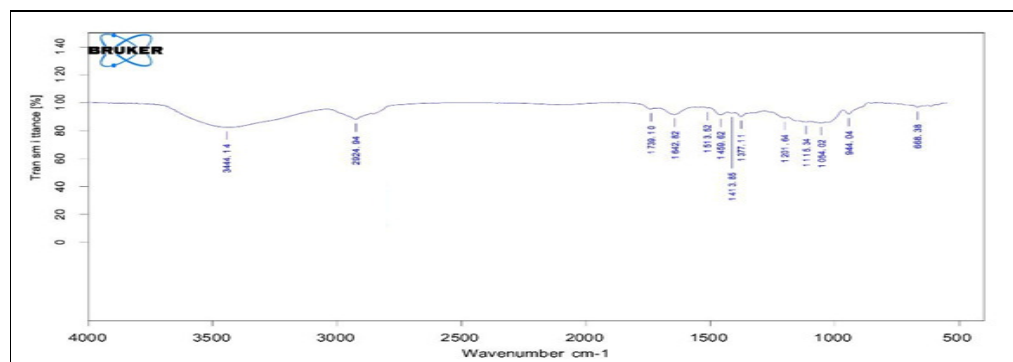
Fig. 10: FTIR Spectrum of Methyl Cellulose
