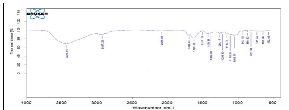
Fig. 11: FTIR Spectrum of Optimized Formulation
